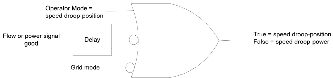
Figure C.1—Droop mode control logic
